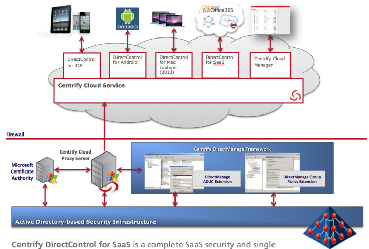
Centrify DirectControl for SaaS is a complete SaaS security and single sign-on solution delivered via the Centrify Cloud Service and supporting hundreds of SaaS applications and providing zero sign-on for mobile applications.
